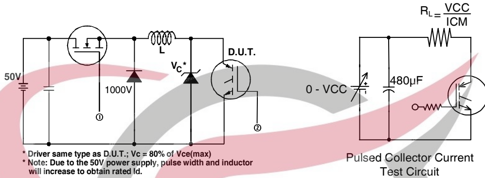
Fig. 13a - Clamped Inductive Load Test Circuit
